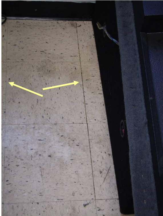
FIGURE 6. Floor tiles near the northeastern corner of the graveyard building. A previous floor crack in this area had been described as having a noticeable movement of “air” coming up through the crack. The floor had been reported to have been redone in the past few years. Even with the passive vapor mitigation system operating, widening of the floor tiles has been noticed where a past floor crack had been located. Compare the tight seem of the tiles on the left to the small gap between the tiles on the right.
